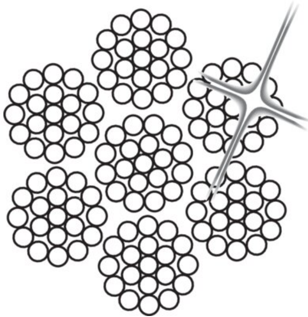
Winch rope
